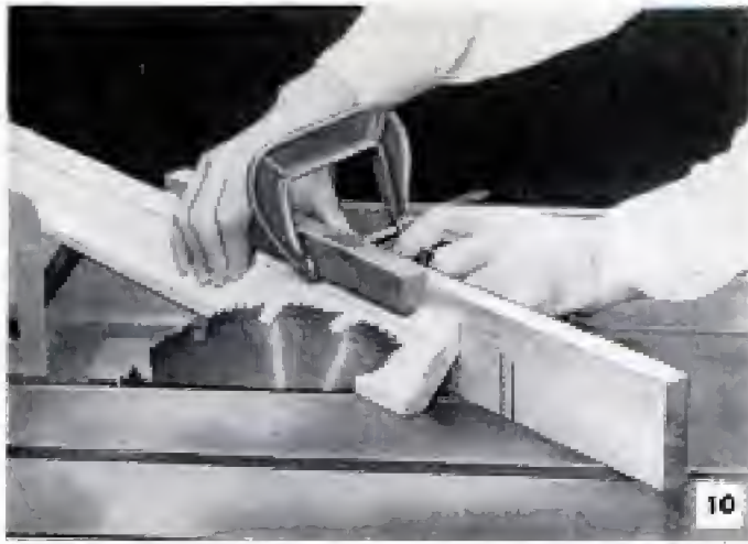
Moldings can be mitered and coped on power tools, using the circular saw for the miter cut and the bandsaw and simple jig for the cope cut
